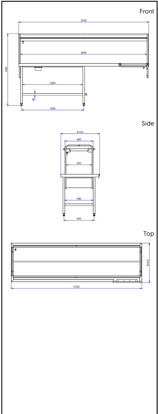
Handling System Sorting Table Left to Right, 2700x800mm
